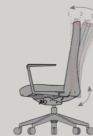
BACK TILT 4 back tilt positions. Tilt angles from 10° at the up-right blocked position up to 30° at the maximum angle
